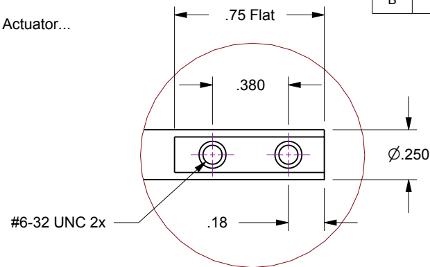
Detail C
