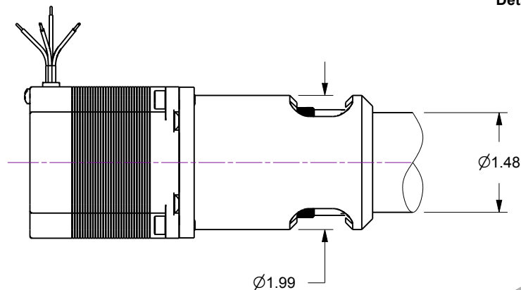
Detail C
